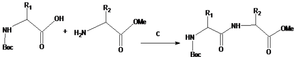
Scheme-iii: General reaction of Dipeptide formation.
