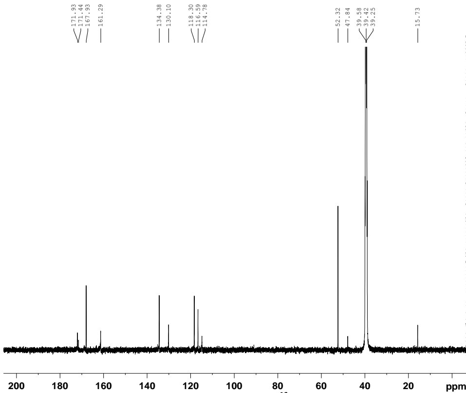
Fig 4: 13 C NMR of ASP 01.
