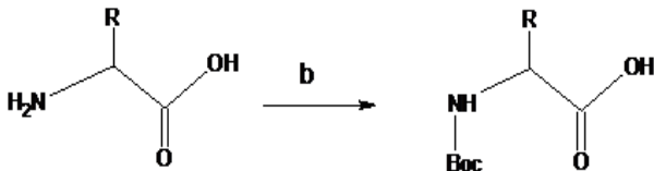
Scheme- ii: General reaction of Boc-amino acid formation.
