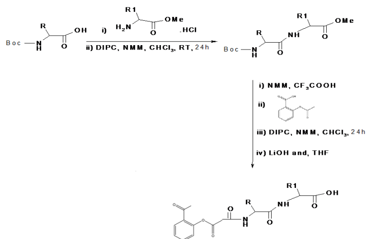
Scheme for Synthesis of Dipeptide containing Aspirin.
