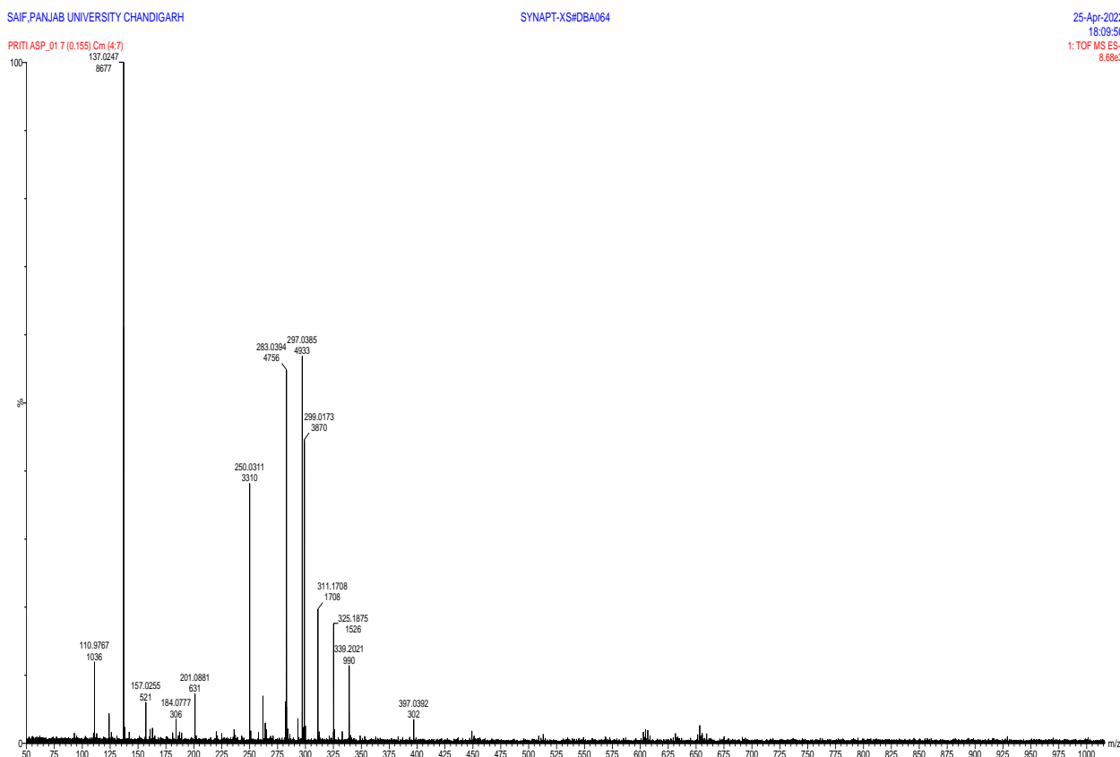
Fig 5: Mass Spectroscopy of ASP 01.
