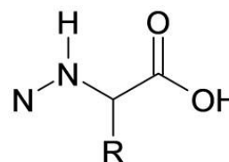
Structure 1: General structure of Amino acid.
