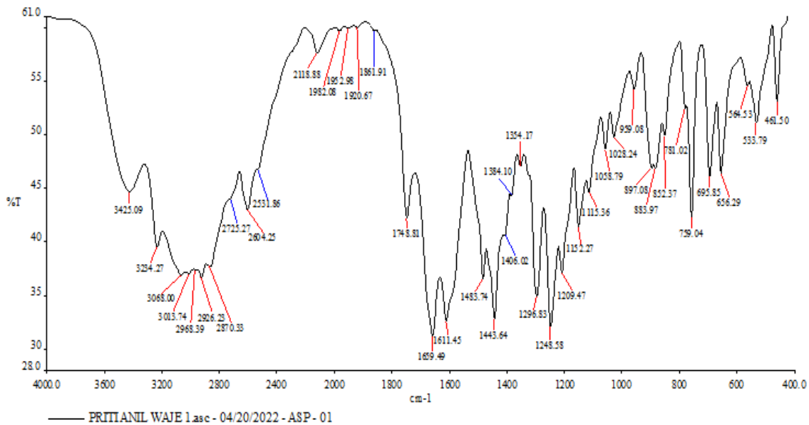
Fig. 1: IR Spectroscopy of Sample ASP 01.
