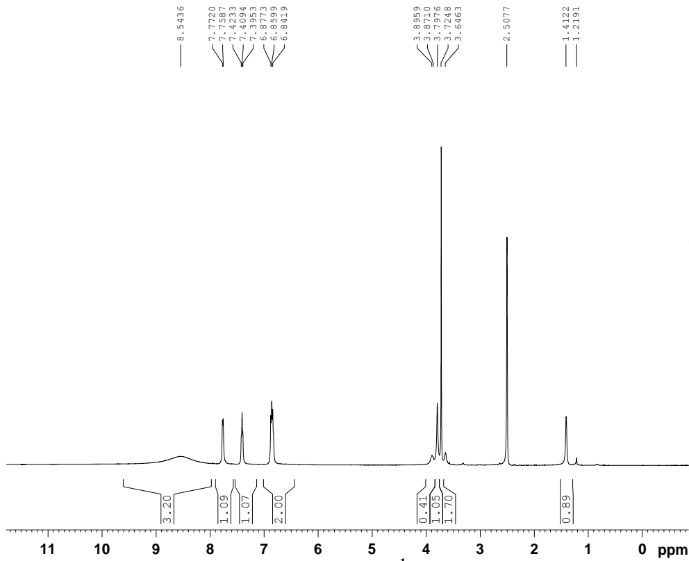
Fig 3: 1 H NMR of ASP 01.
