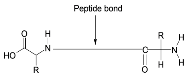
Structure 2: Structure of Peptide bond.
