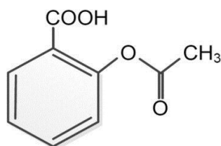
Structure 4: Structure of Aspirin.
