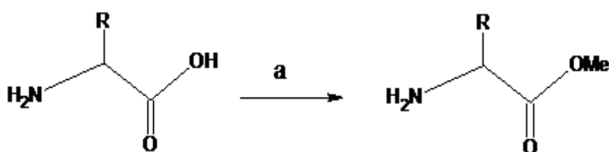
Scheme i: General reaction of Ester formation.
