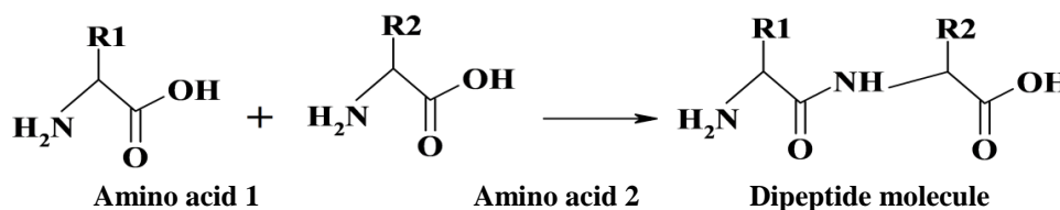
Structure 3: Structure of Dipeptide.
