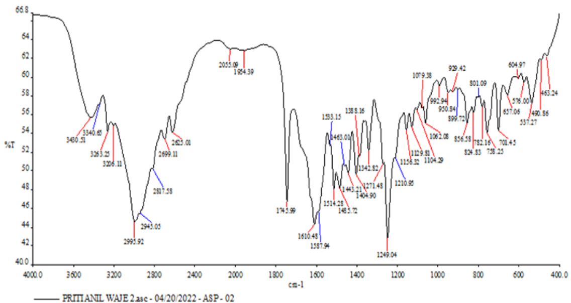
Fig. 2: IR Spectroscopy of Sample ASP 02.
