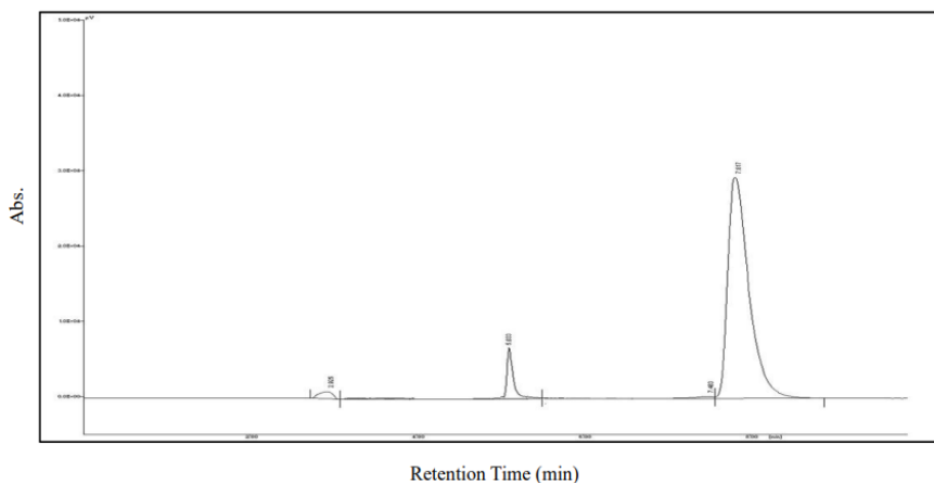
Fig. 8: Chromatogram of Ivabradine (100 \mu\text{g/ml} ) after alkaline hydrolysis.
