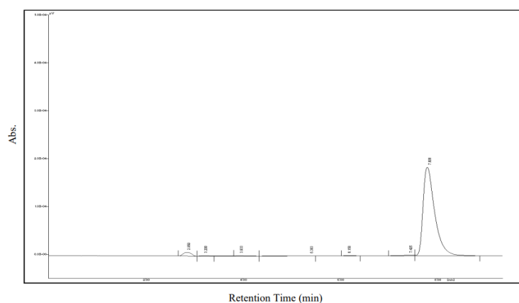
Fig. 12: Chromatogram of Ivabradine (10 µg/ml) after oxidation.
